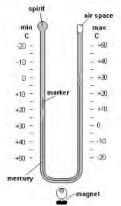
Figure 2. The maximum-minimum thermometer
